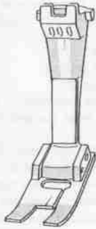
Zigzag foot 000 Needle: 80-70 Thread: 30
